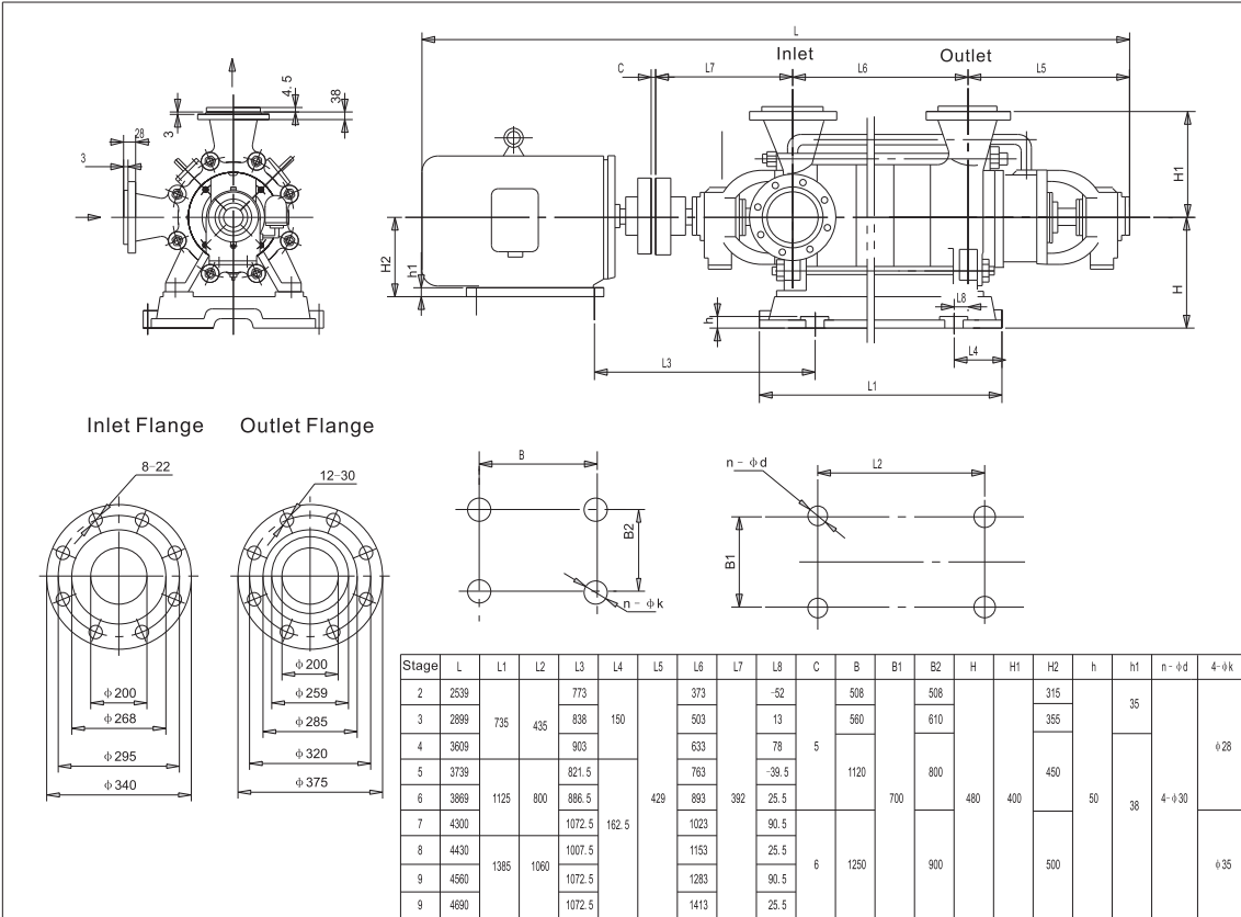
HMC280-65 Overall Dimension Drawing
