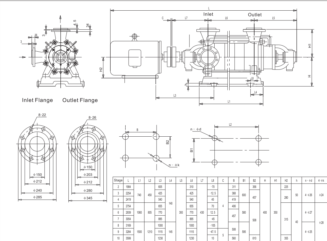
HMC155-67 Overall Dimension Drawing
